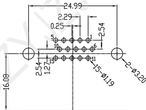
RECOMMENED PCB LAYOUT TOP VIEW (TOLERANCE:±0.05)
